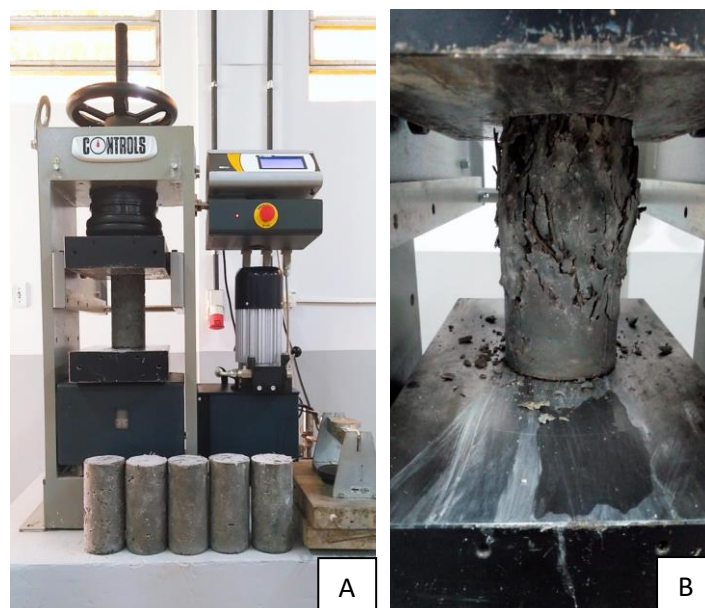
Figure 5: (A) Test of resistance to compression, (B) Uniaxial compression.
