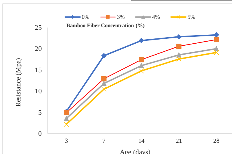
Figure 6: Graph of compressive strength gains after 3, 7, 14, 21 and 28 days with addition of 5 cm bamboo fiber concentration.
