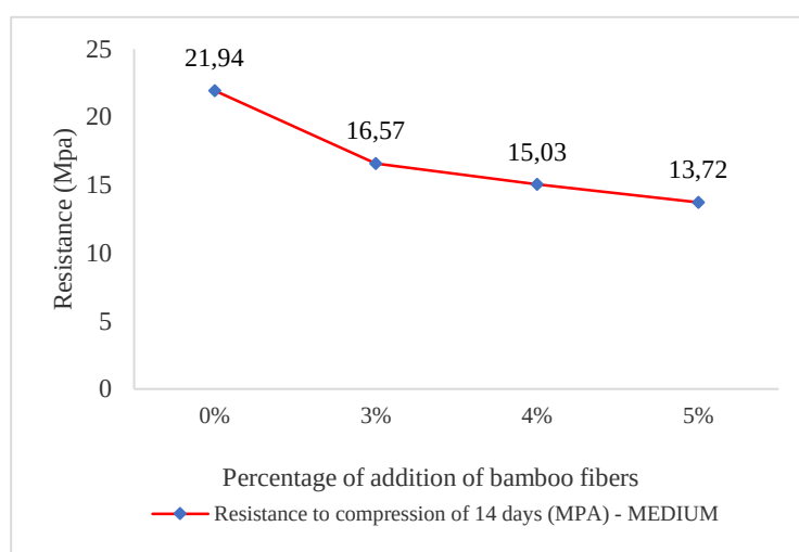
Figure 8: Graph of resistance to compression for 14 days.
