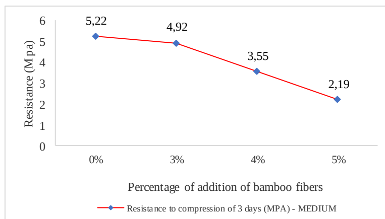
Figure 7: Graph of resistance to compression for 3 days.
