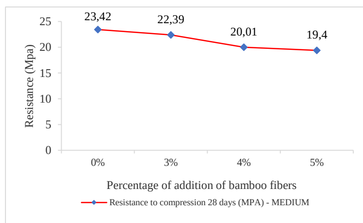
Figure 9: Graph of resistance to compression for 28 days.
