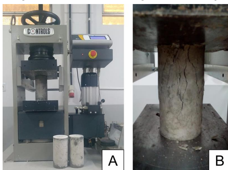
Figure 4: (A) Test of resistance to compression, (B) Uniaxial compression
