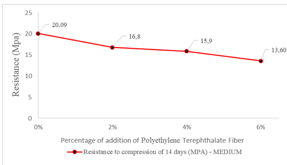
Figure7: Graph of resistance to compression for 14 days.
