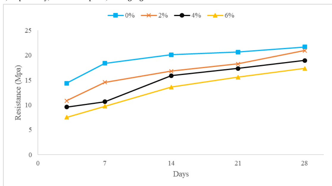
Figure 5: Graph of compressive strength gains after 3, 7, 14, 21 and 28 days with addition of 5 cm bamboo fiber concentration.
