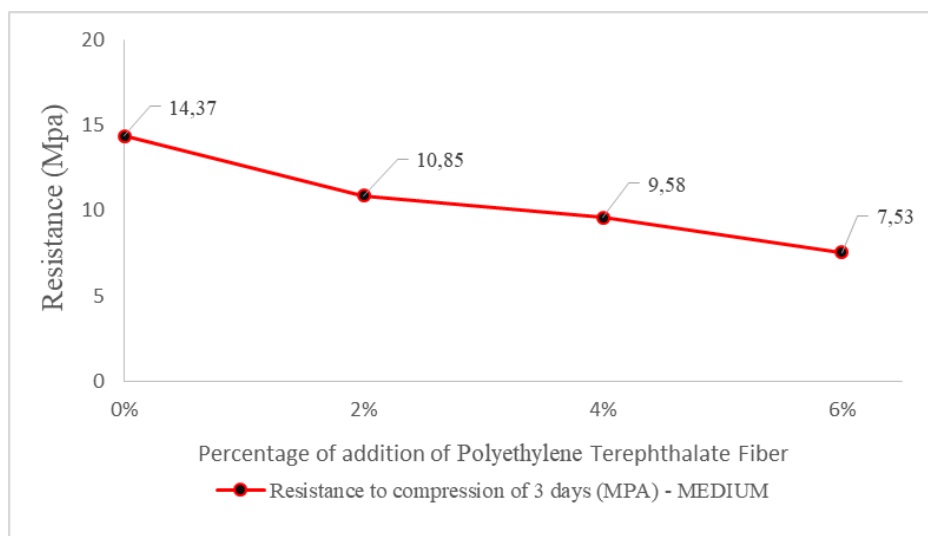
Figure 6: Graph of resistance to compression for 3 days.
