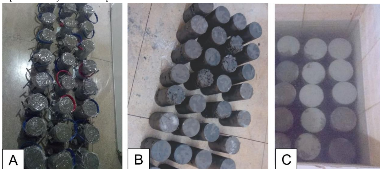
Figure 3: PC molding and demolding process (A) formation of evidence bodies, (B) removal of evidence bodies, (C) hydration and cure of bodies of evidence.
