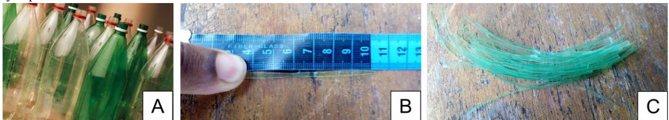
Figure 1: (A) PET bottles used in fiber manufacture, (B) manual fiber measurement, (C) fibers already cut and ready for use.
